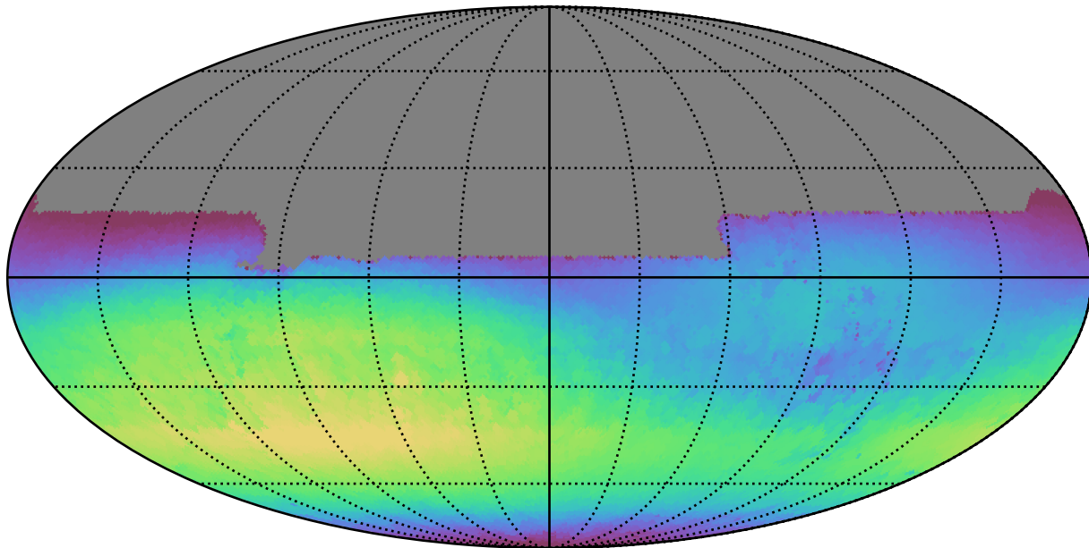
ddf_loaded_fl8_v3.4_10yrs All sky u band: Max skyBrightness
