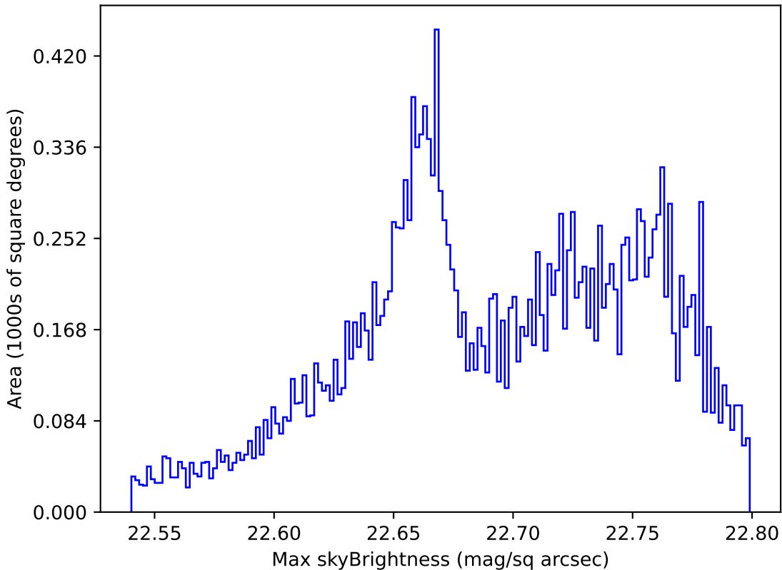
ddf_loaded_fl8_v3.4_10yrs All sky u band: Max skyBrightness
