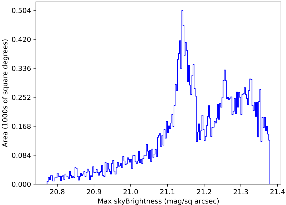
ddf_loaded_fl8_v3.4_10yrs All sky r band: Max skyBrightness
