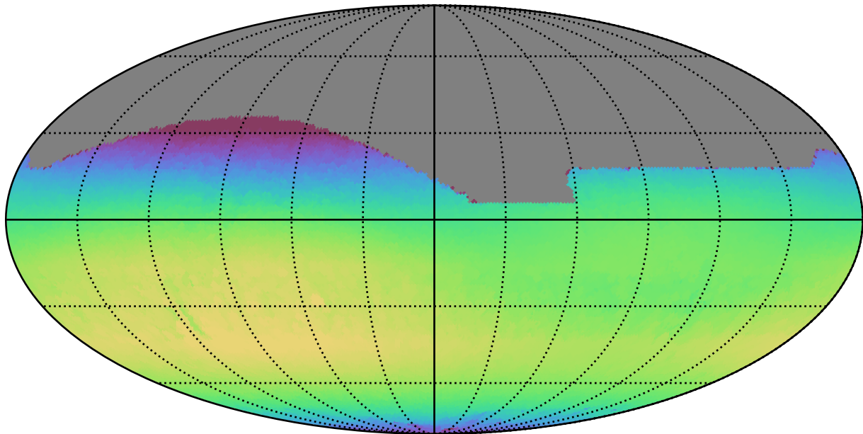
ddf_loaded_fl8_v3.4_10yrs All sky i band: Max skyBrightness
