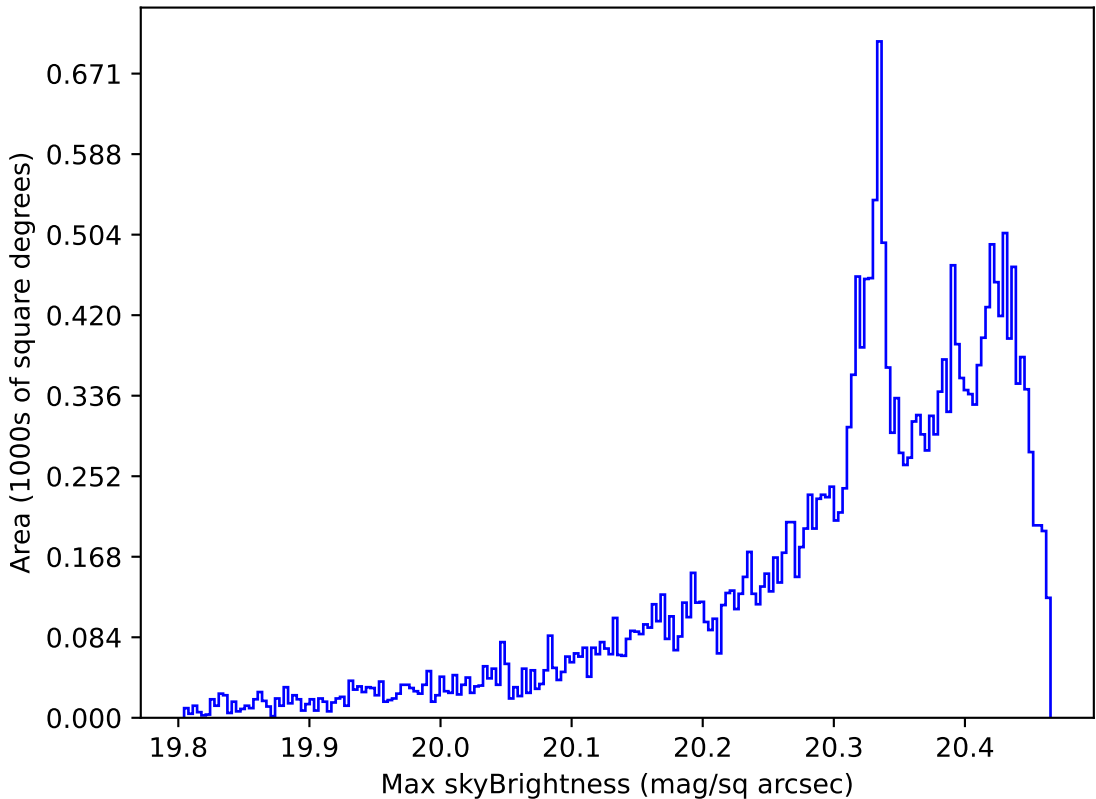
ddf_loaded_fl8_v3.4_10yrs All sky i band: Max skyBrightness
