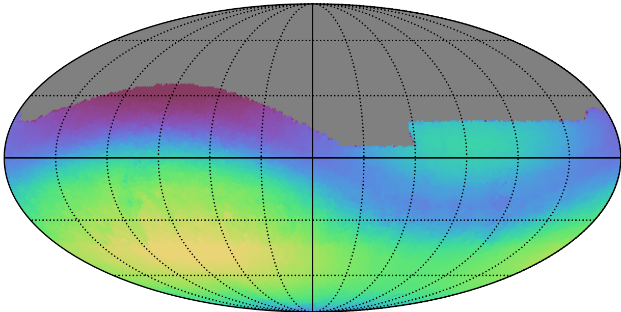
ddf_loaded_fl8_v3.4_10yrs All sky g band: Max skyBrightness
