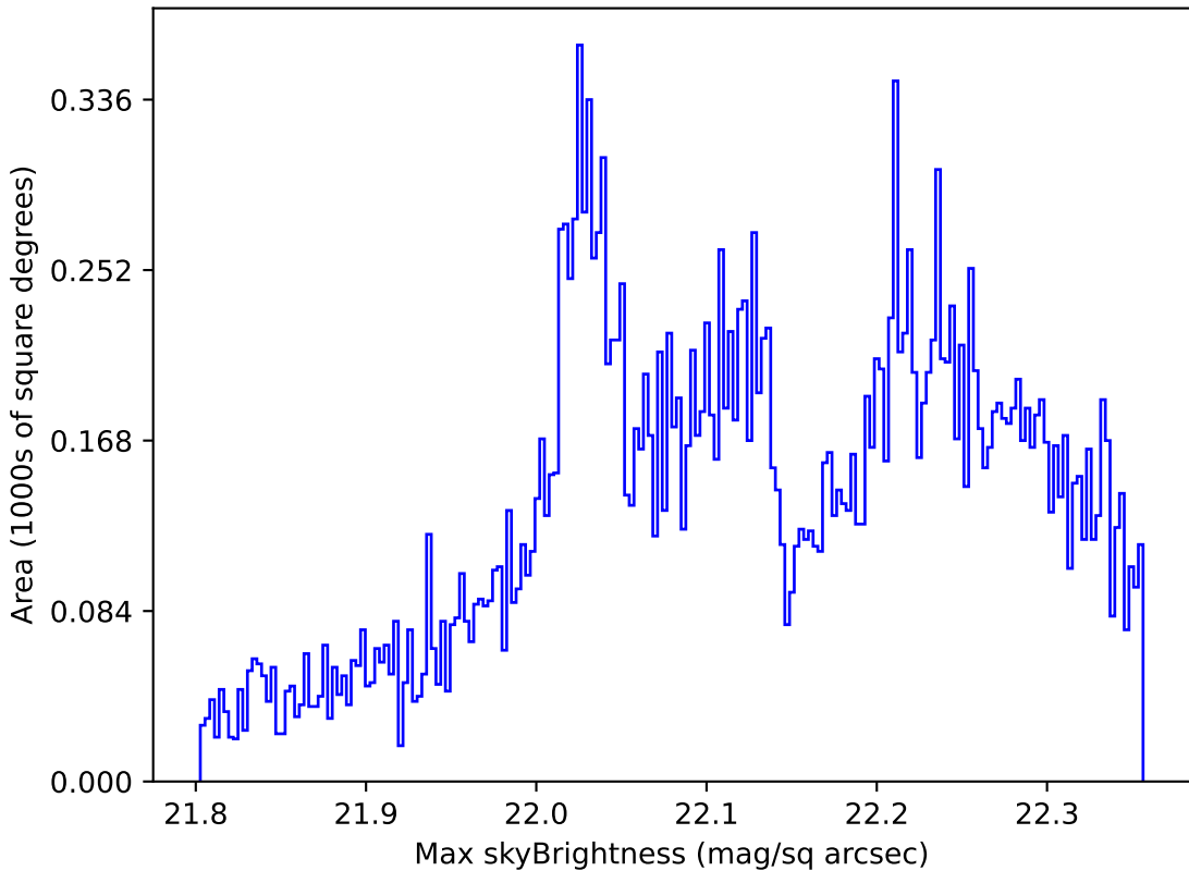
ddf_loaded_fl8_v3.4_10yrs All sky g band: Max skyBrightness
