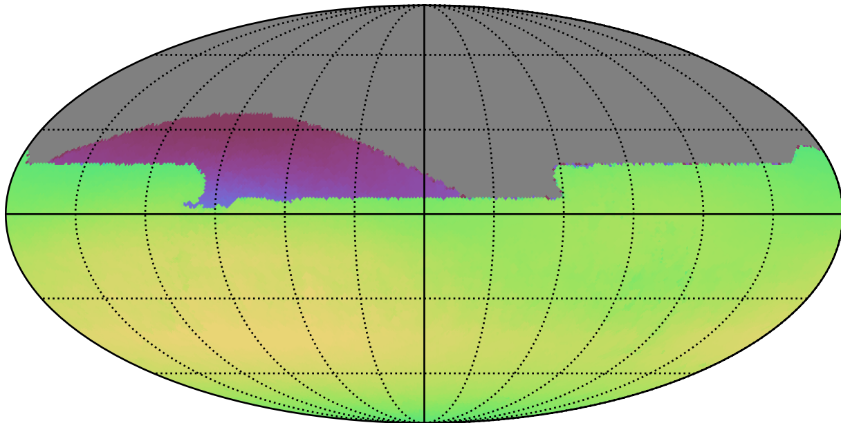
ddf_loaded_fl8_v3.4_10yrs All sky all bands: Max skyBrightness
