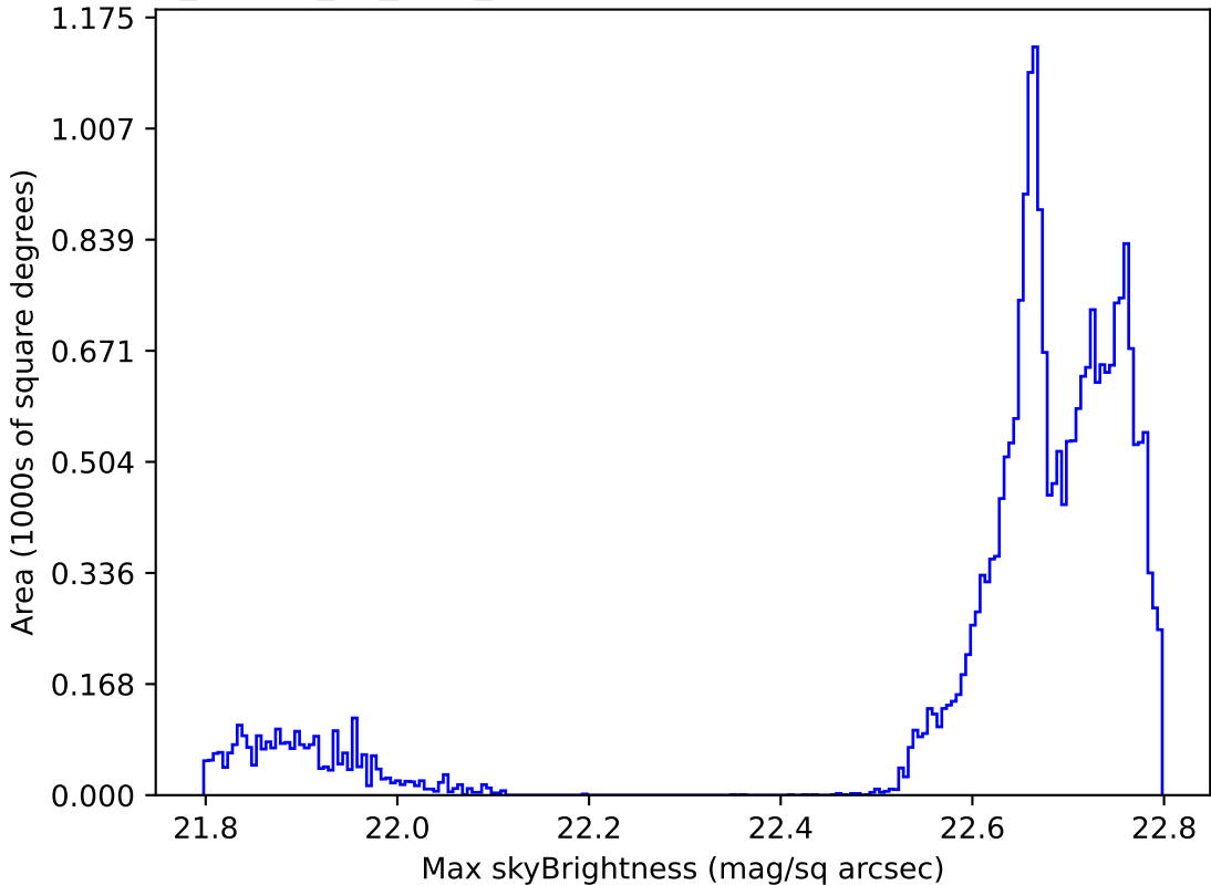
ddf_loaded_fl8_v3.4_10yrs All sky all bands: Max skyBrightness
