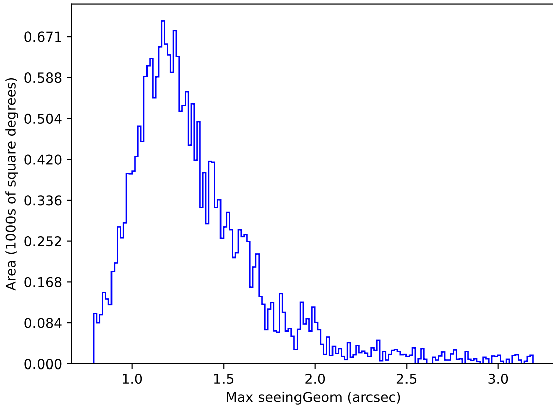
ddf_loaded_fl8_v3.4_10yrs Yr 1 u band: Max seeingGeom
