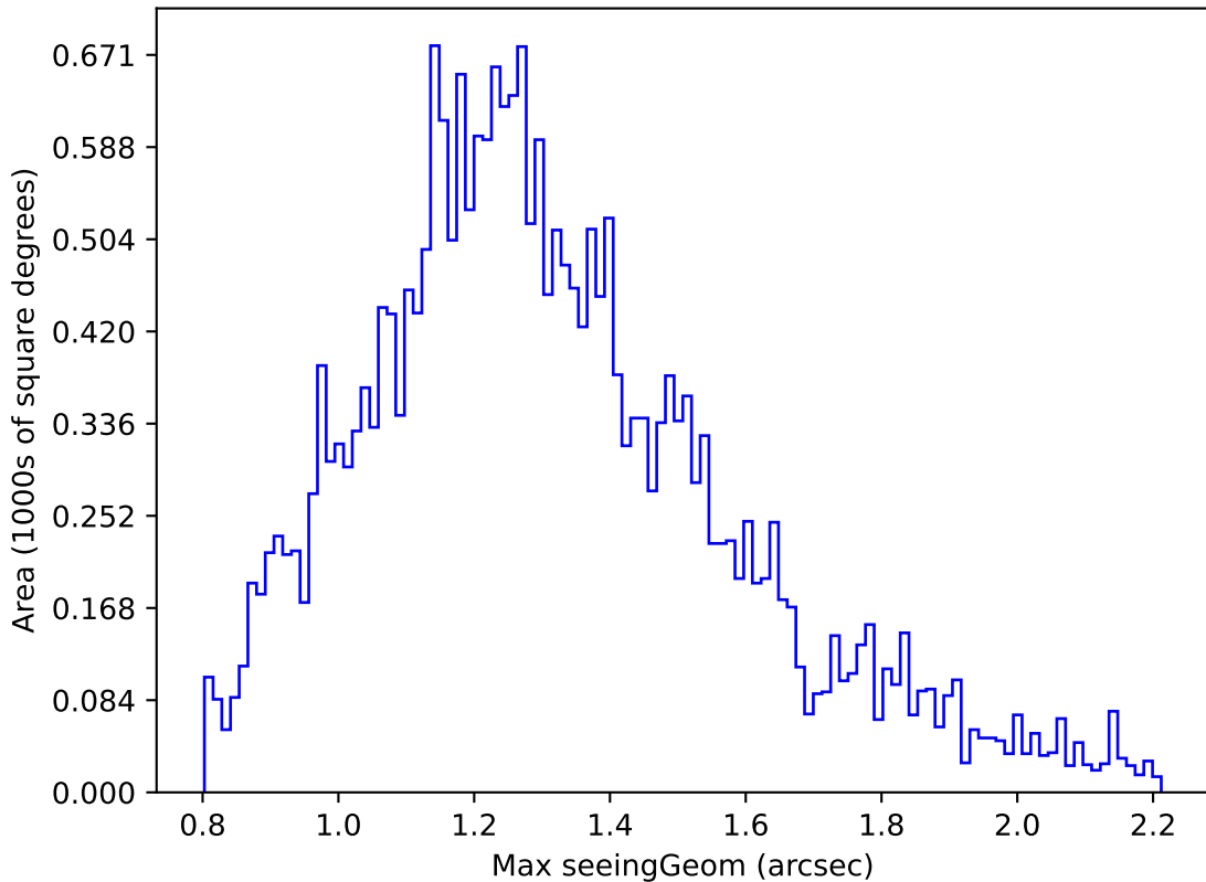
ddf_loaded_fl8_v3.4_10yrs Yr 1 r band: Max seeingGeom
