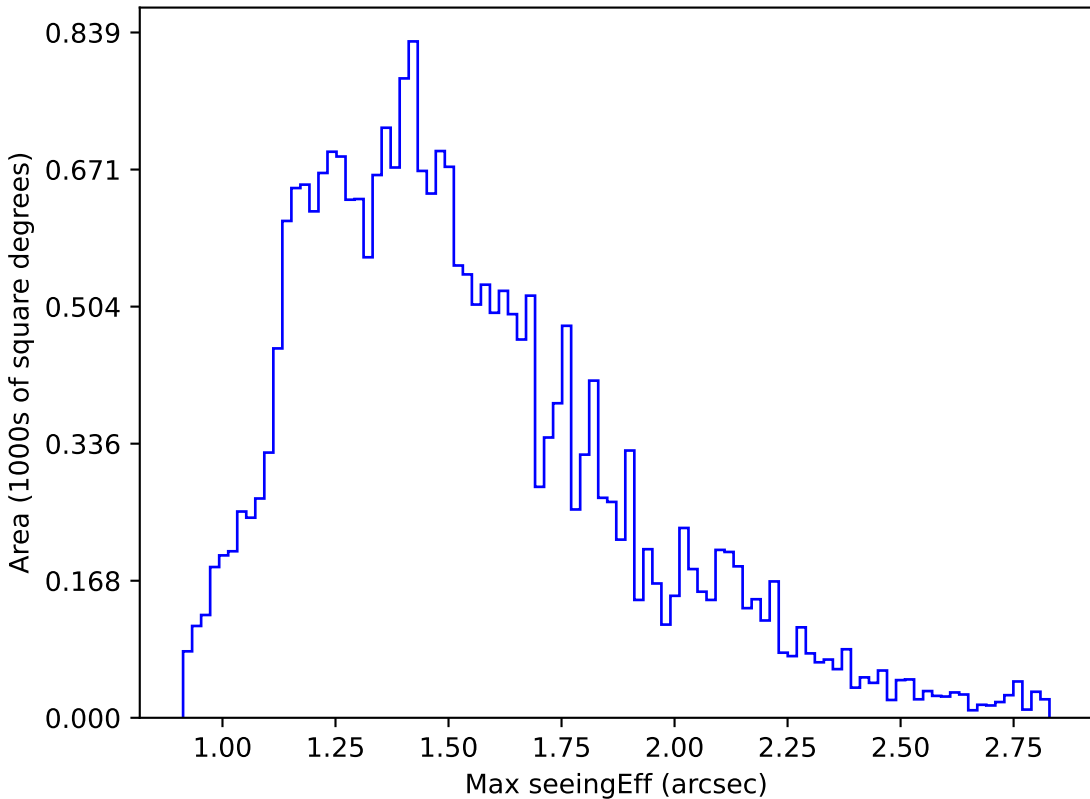
ddf_loaded_fl8_v3.4_10yrs Yr 1 z band: Max seeingEff
