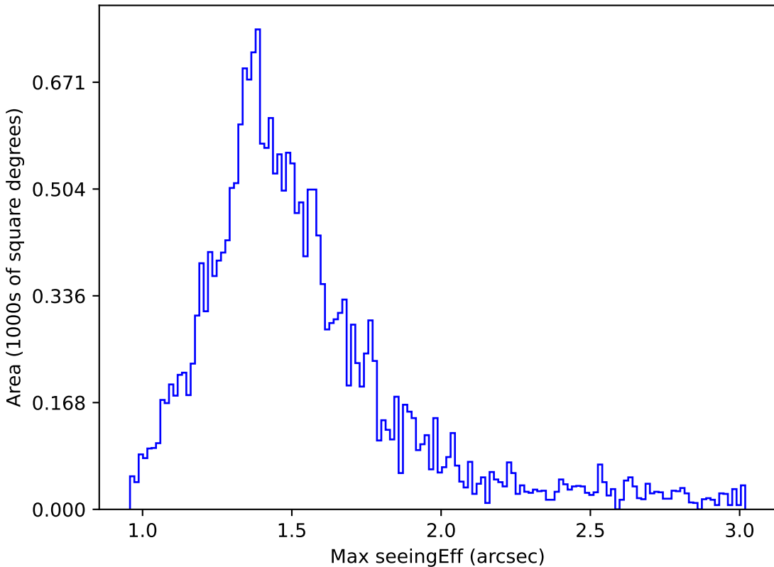
ddf_loaded_fl8_v3.4_10yrs Yr 1 y band: Max seeingEff
