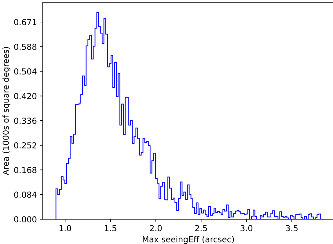
ddf_loaded_fl8_v3.4_10yrs Yr 1 u band: Max seeingEff
