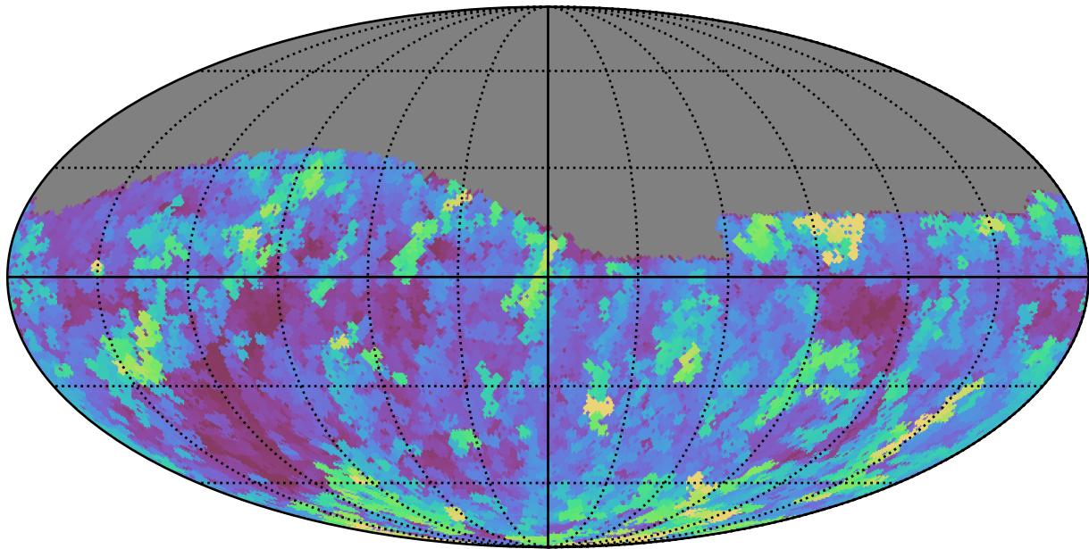
ddf_loaded_fl8_v3.4_10yrs Yr 1 r band: Max seeingEff
