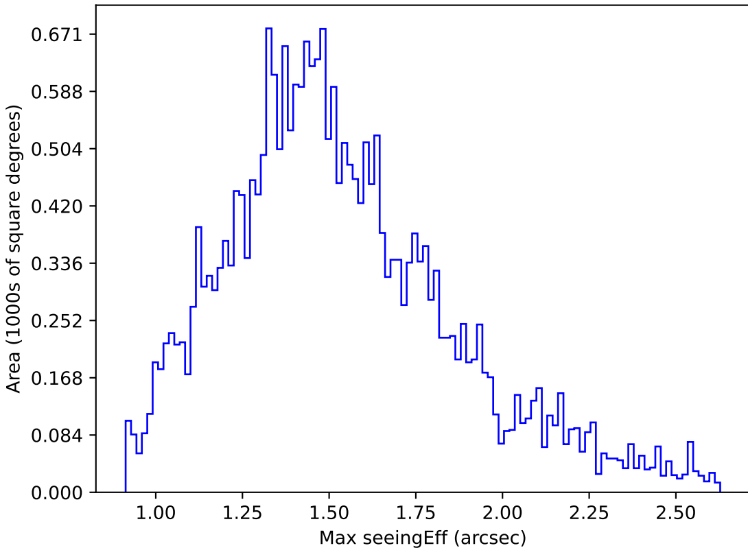
ddf_loaded_fl8_v3.4_10yrs Yr 1 r band: Max seeingEff
