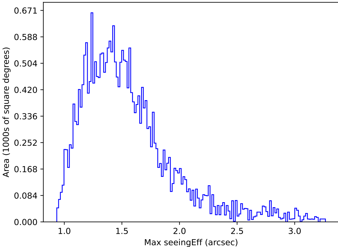
ddf_loaded_fl8_v3.4_10yrs Yr 1 i band: Max seeingEff
