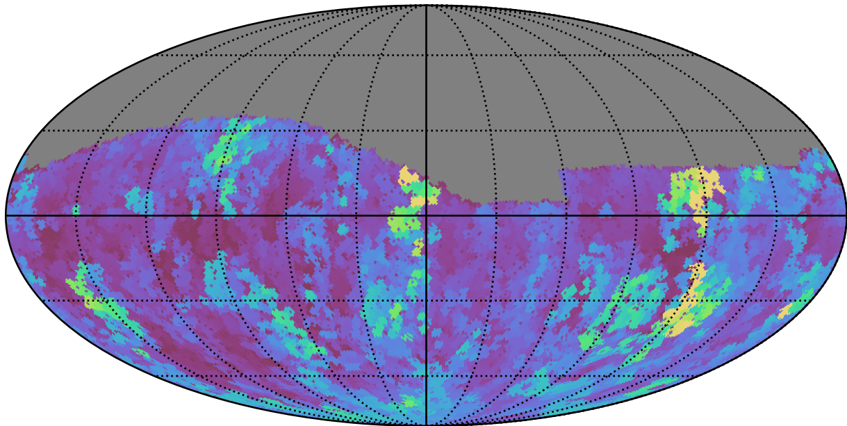
ddf_loaded_fl8_v3.4_10yrs Yr 1 g band: Max seeingEff
