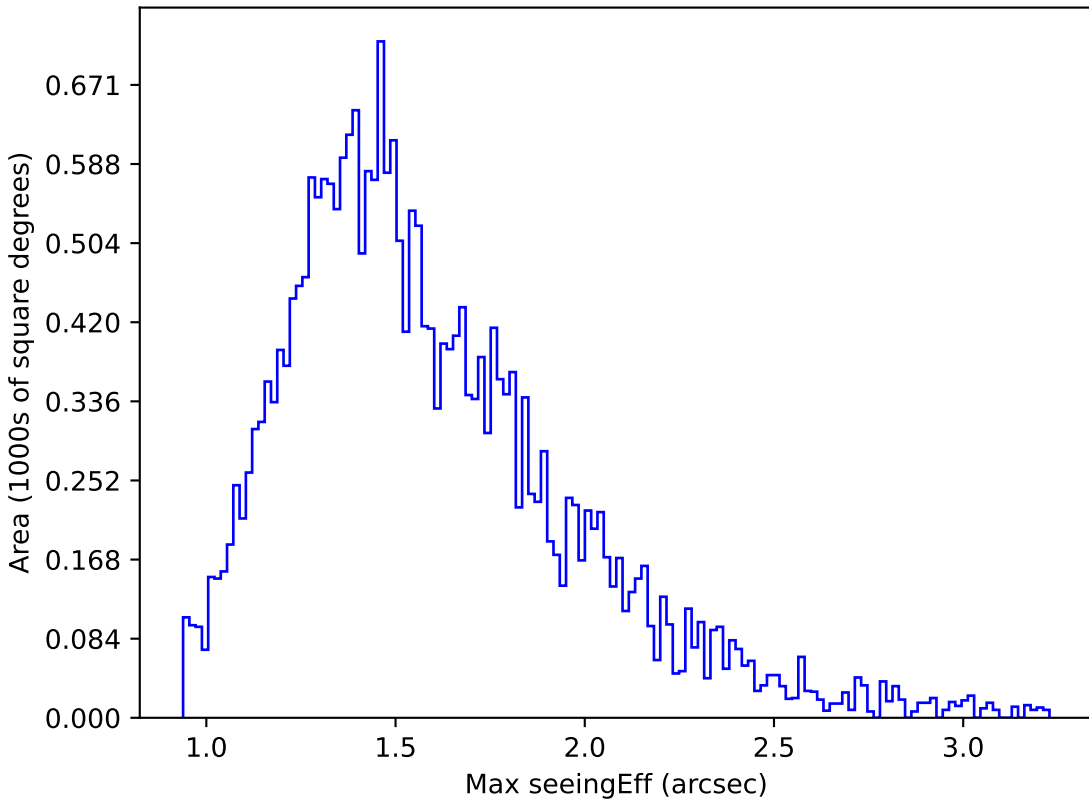
ddf_loaded_fl8_v3.4_10yrs Yr 1 g band: Max seeingEff
