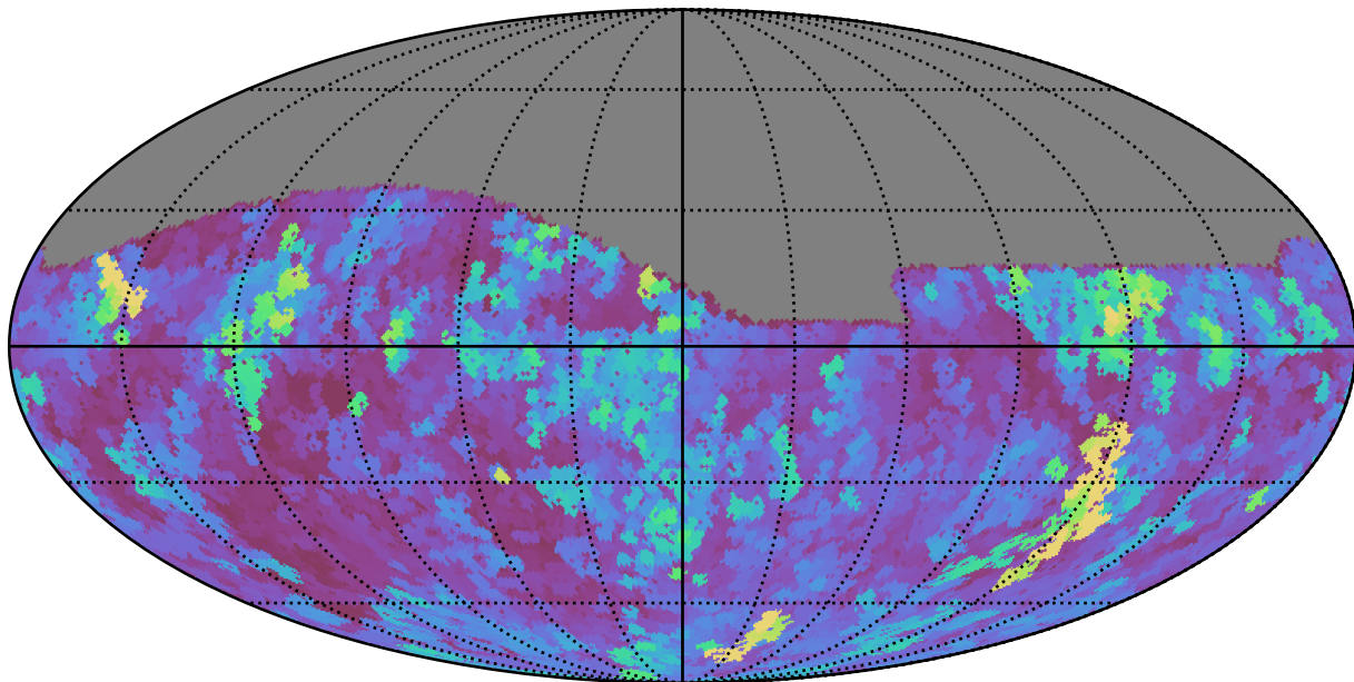
ddf_loaded_fl8_v3.4_10yrs Yr 1 all bands: Max seeingEff
