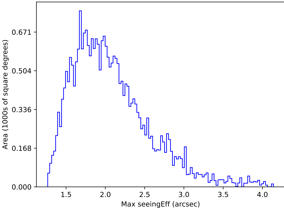
ddf_loaded_fl8_v3.4_10yrs Yr 1 all bands: Max seeingEff
