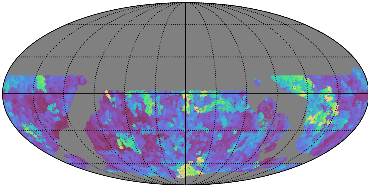
ddf_loaded_fl8_v3.4_10yrs WFD z band: Max seeingEff
