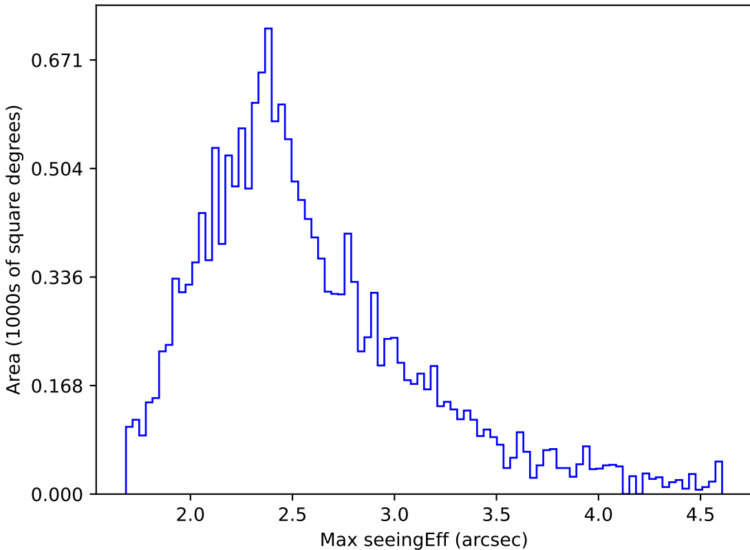
ddf_loaded_fl8_v3.4_10yrs WFD z band: Max seeingEff
