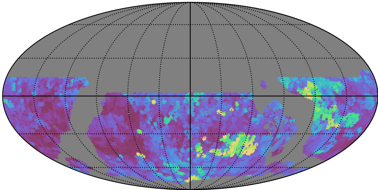
ddf_loaded_fl8_v3.4_10yrs WFD y band: Max seeingEff
