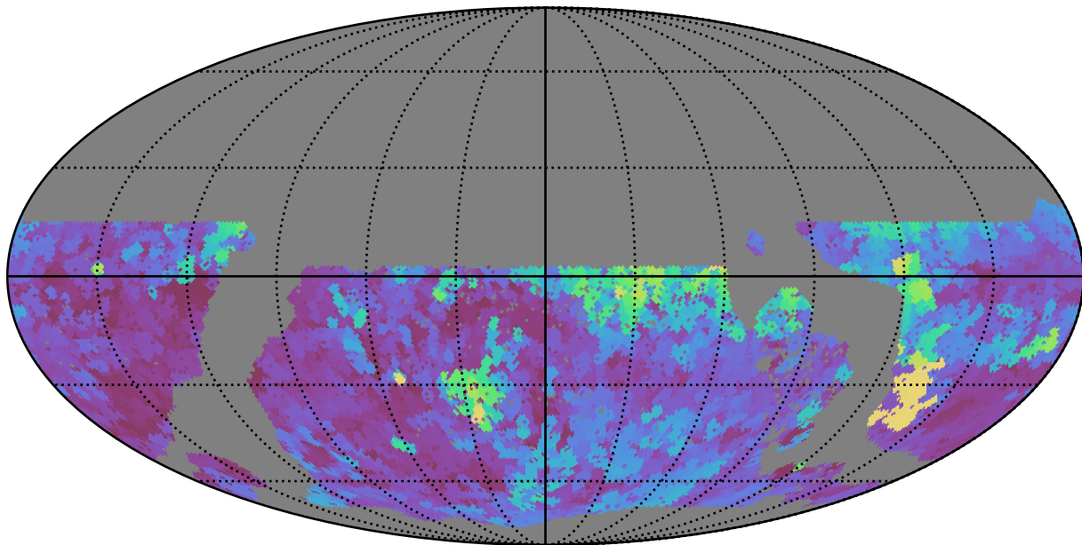
ddf_loaded_fl8_v3.4_10yrs WFD u band: Max seeingEff
