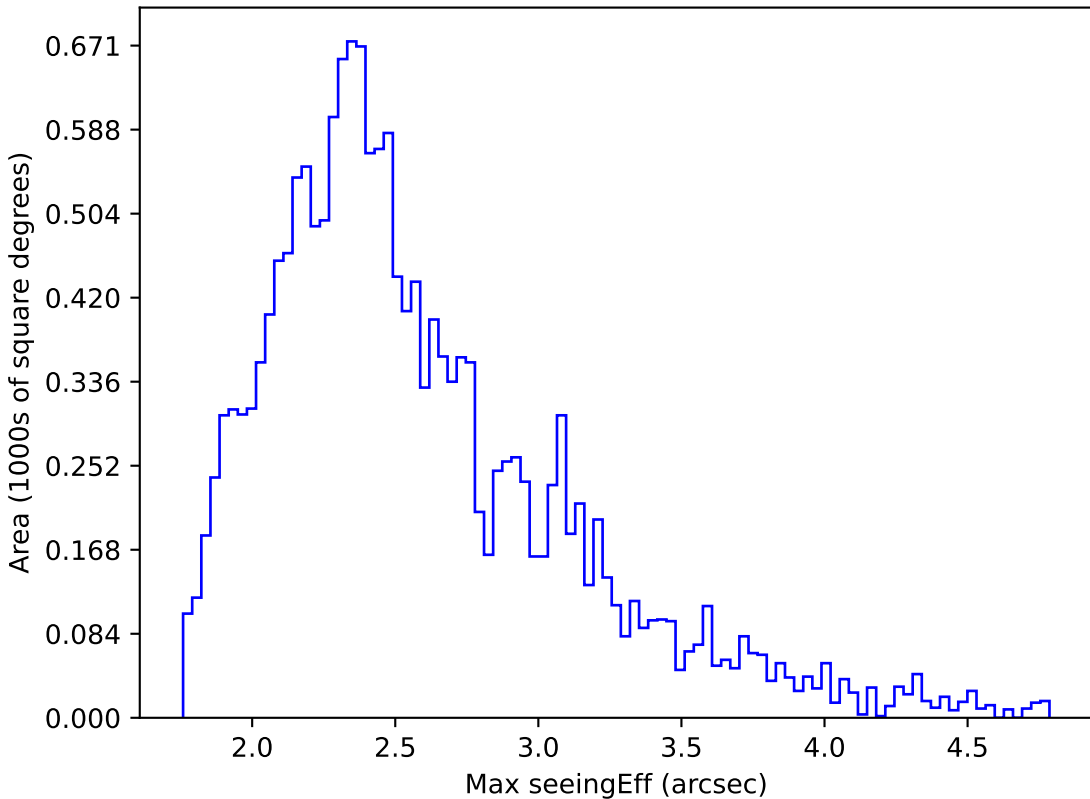
ddf_loaded_fl8_v3.4_10yrs WFD u band: Max seeingEff
