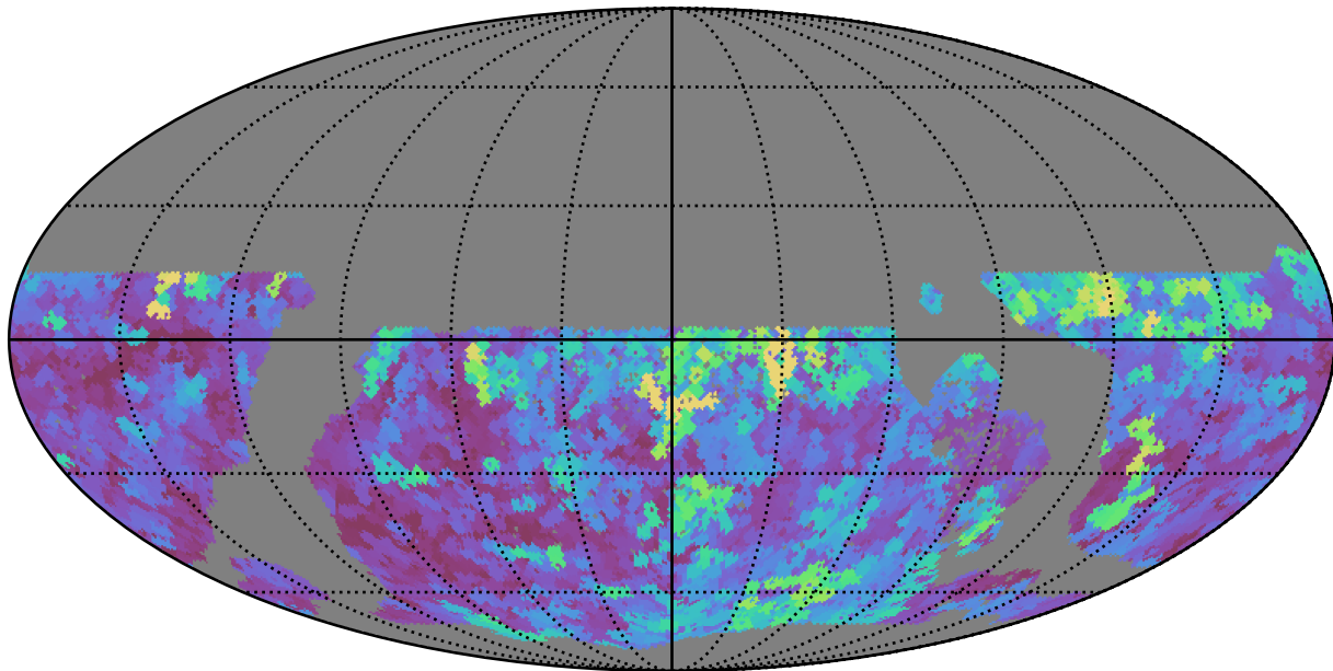
ddf_loaded_fl8_v3.4_10yrs WFD r band: Max seeingEff
