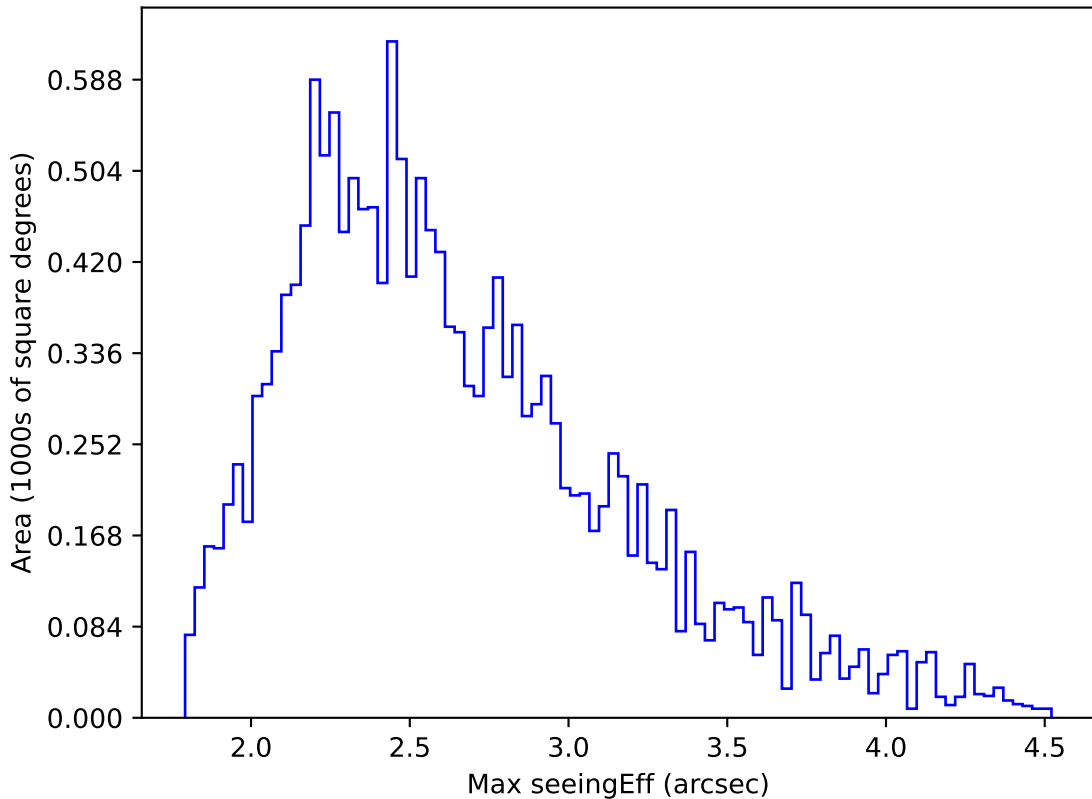
ddf_loaded_fl8_v3.4_10yrs WFD r band: Max seeingEff
