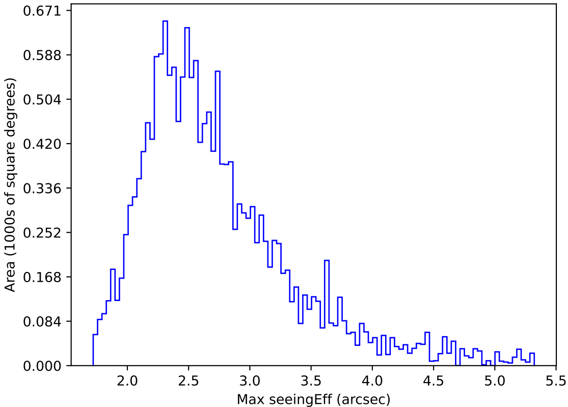
ddf_loaded_fl8_v3.4_10yrs WFD i band: Max seeingEff
