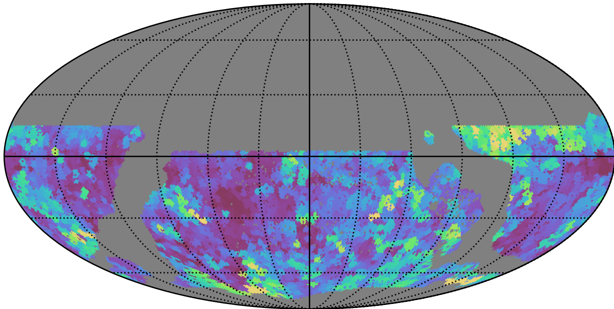
ddf_loaded_fl8_v3.4_10yrs WFD g band: Max seeingEff
