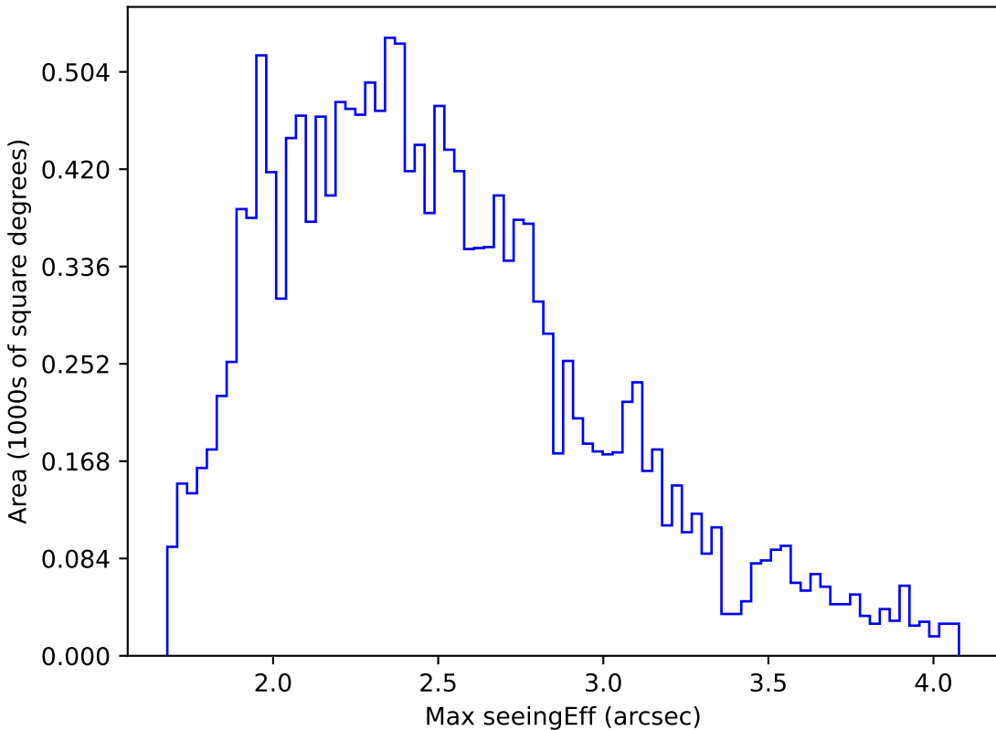
ddf_loaded_fl8_v3.4_10yrs WFD g band: Max seeingEff
