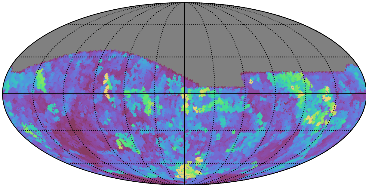
ddf_loaded_fl8_v3.4_10yrs All sky z band: Max seeingEff
