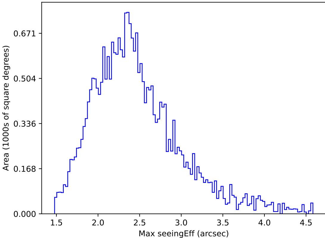
ddf_loaded_fl8_v3.4_10yrs All sky z band: Max seeingEff
