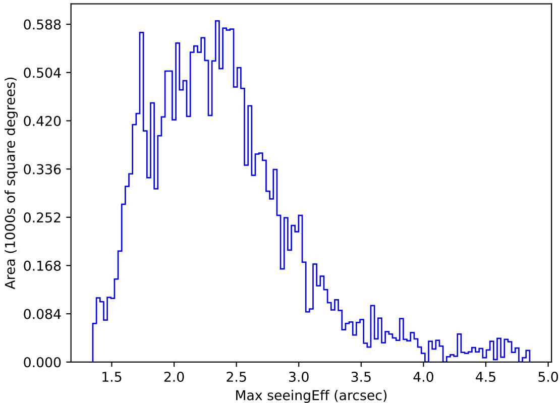
ddf_loaded_fl8_v3.4_10yrs All sky y band: Max seeingEff
