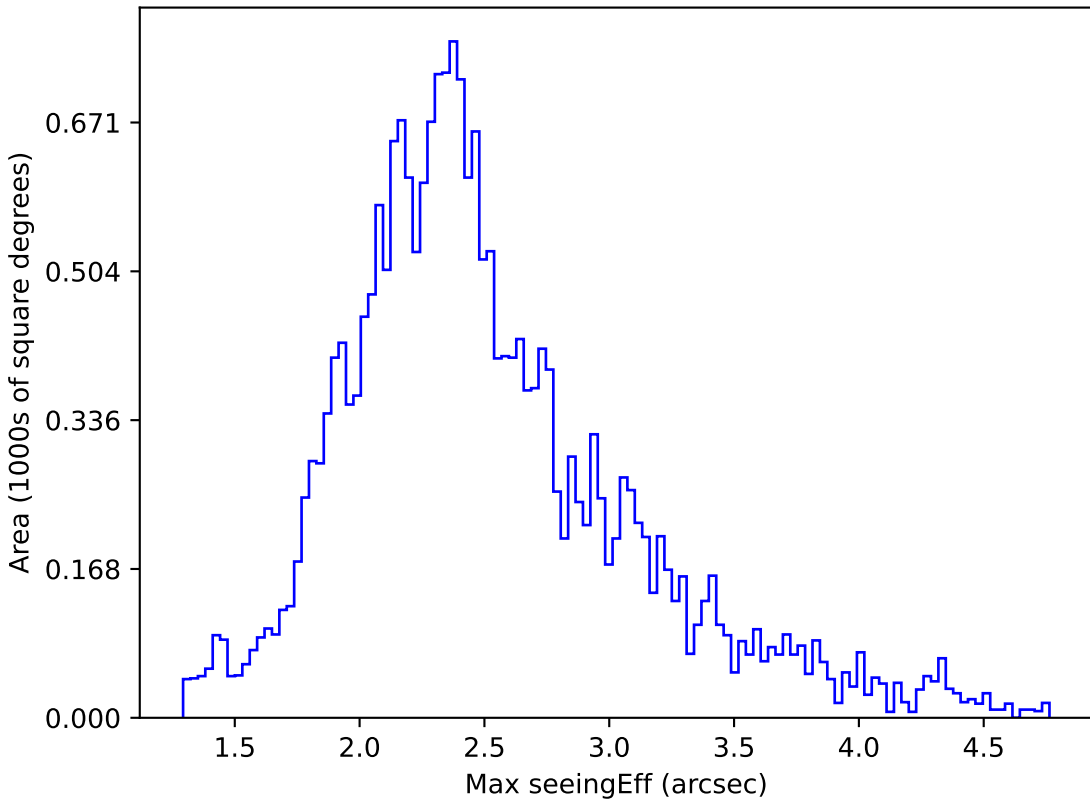
ddf_loaded_fl8_v3.4_10yrs All sky u band: Max seeingEff
