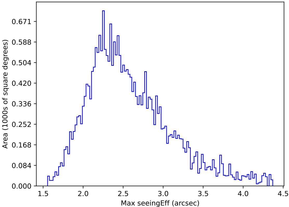
ddf_loaded_fl8_v3.4_10yrs All sky r band: Max seeingEff
