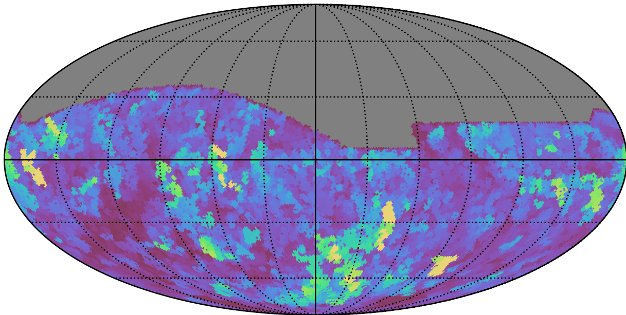
ddf_loaded_fl8_v3.4_10yrs All sky i band: Max seeingEff
