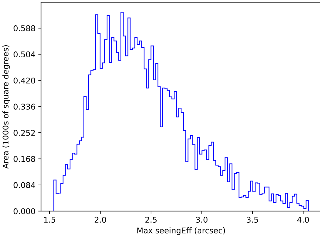
ddf_loaded_fl8_v3.4_10yrs All sky g band: Max seeingEff
