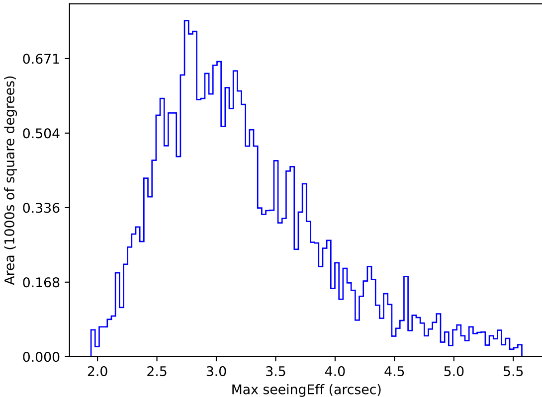
ddf_loaded_fl8_v3.4_10yrs All sky all bands: Max seeingEff
