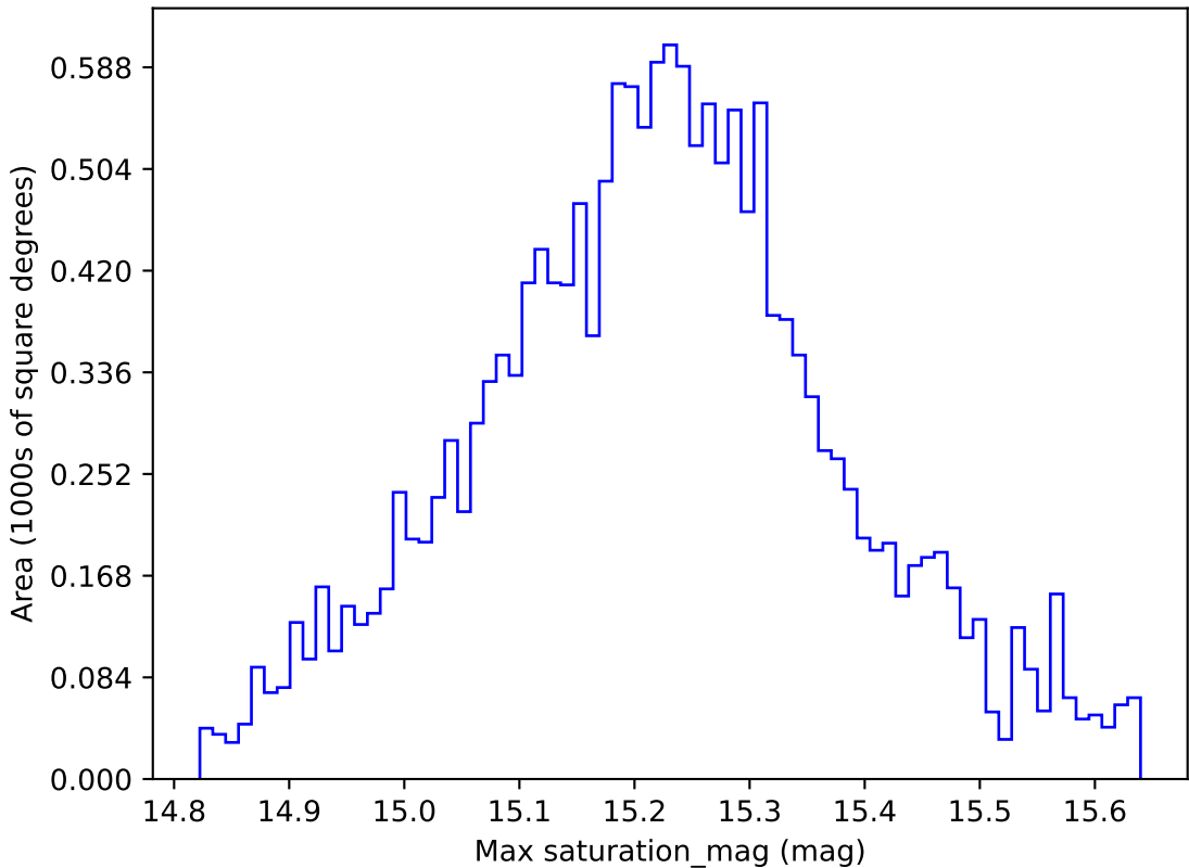
ddf_loaded_fl8_v3.4_10yrs WFD z band: Max saturation_mag
