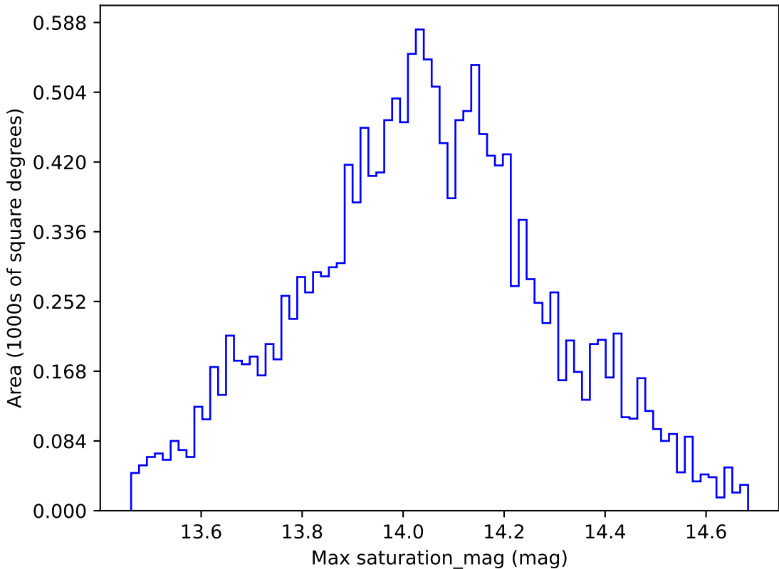
ddf_loaded_fl8_v3.4_10yrs WFD u band: Max saturation_mag
