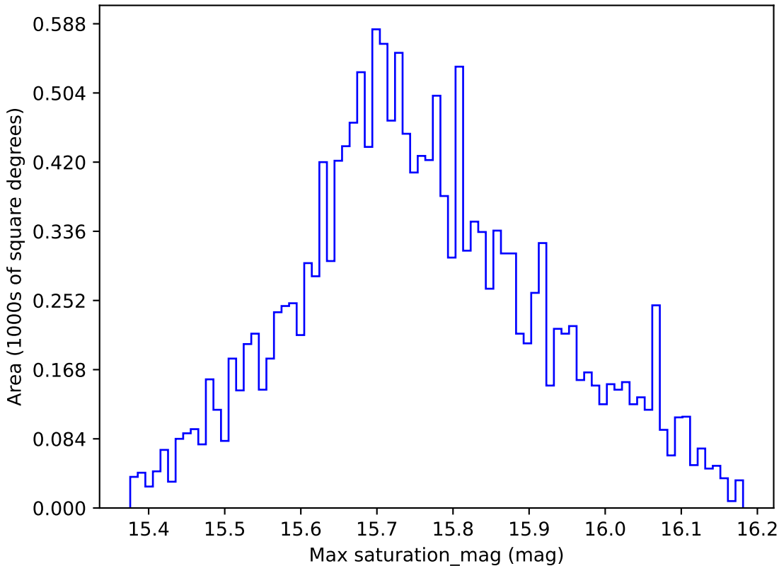
ddf_loaded_fl8_v3.4_10yrs WFD r band: Max saturation_mag
