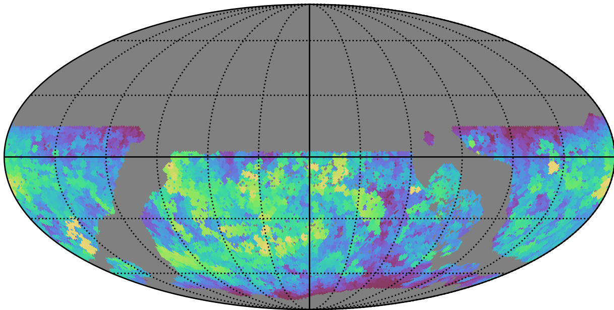
ddf_loaded_fl8_v3.4_10yrs WFD g band: Max saturation_mag
