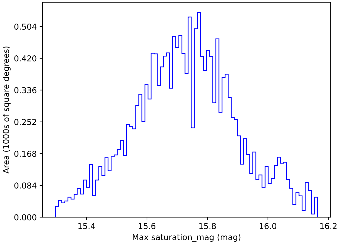
ddf_loaded_fl8_v3.4_10yrs WFD g band: Max saturation_mag
