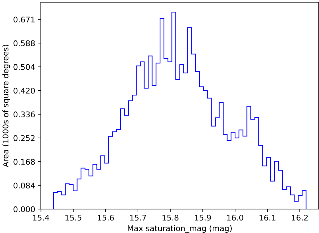
ddf_loaded_fl8_v3.4_10yrs WFD all bands: Max saturation_mag
