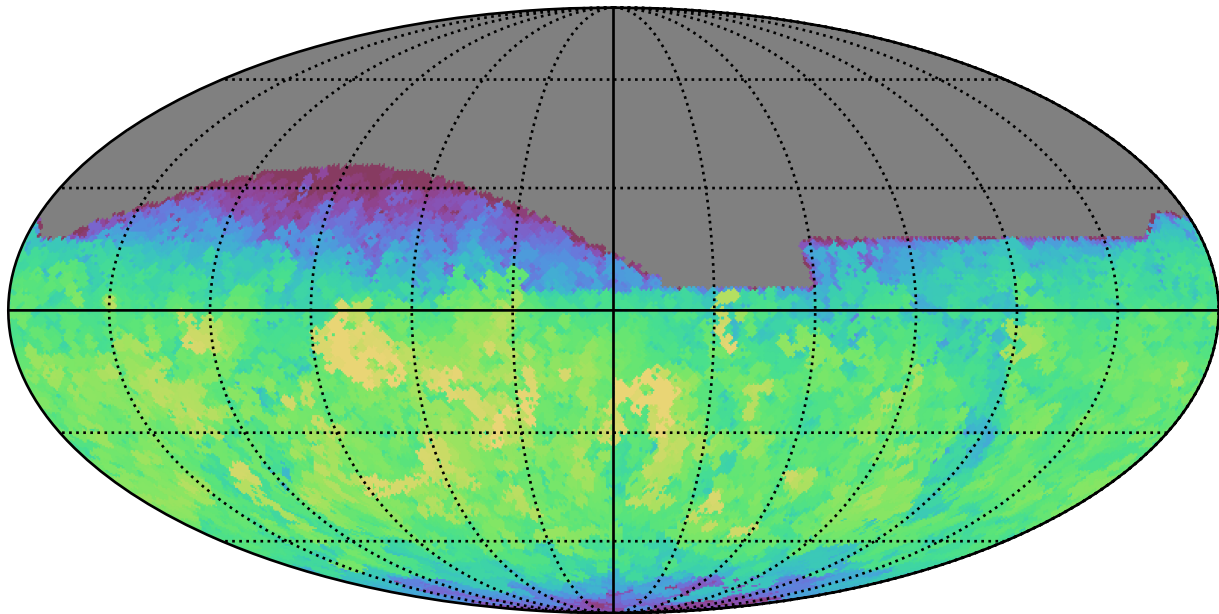
ddf_loaded_fl8_v3.4_10yrs All sky z band: Max saturation_mag
