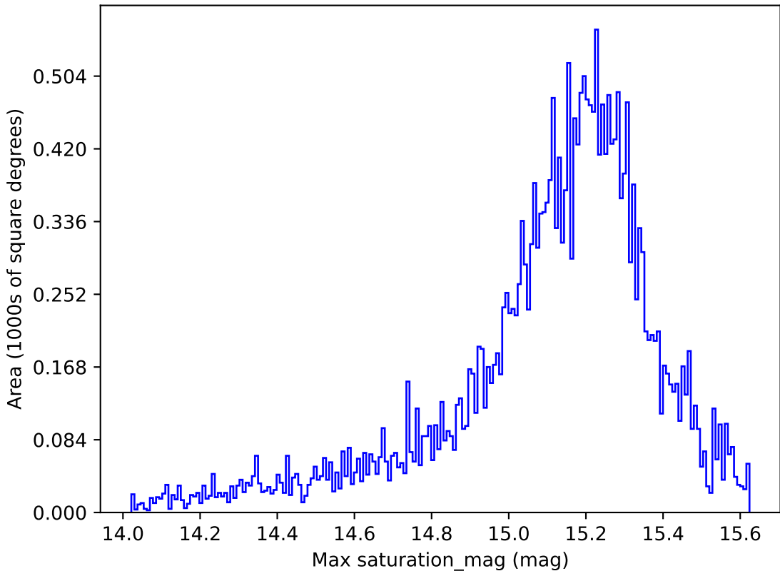
ddf_loaded_fl8_v3.4_10yrs All sky z band: Max saturation_mag
