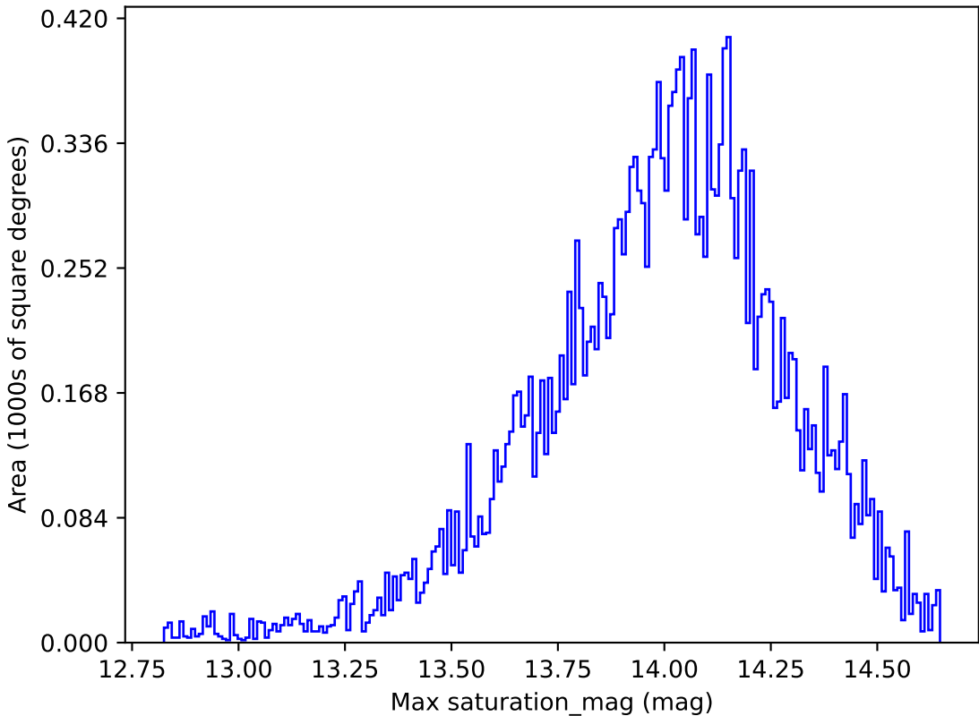
ddf_loaded_fl8_v3.4_10yrs All sky u band: Max saturation_mag
