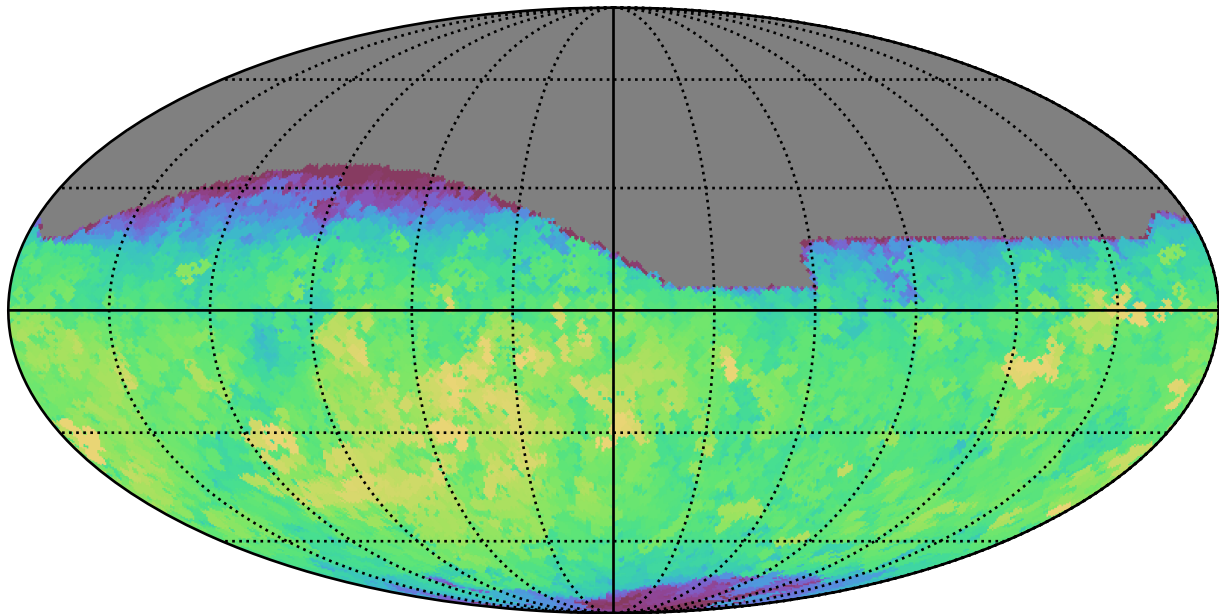
ddf_loaded_fl8_v3.4_10yrs All sky r band: Max saturation_mag
