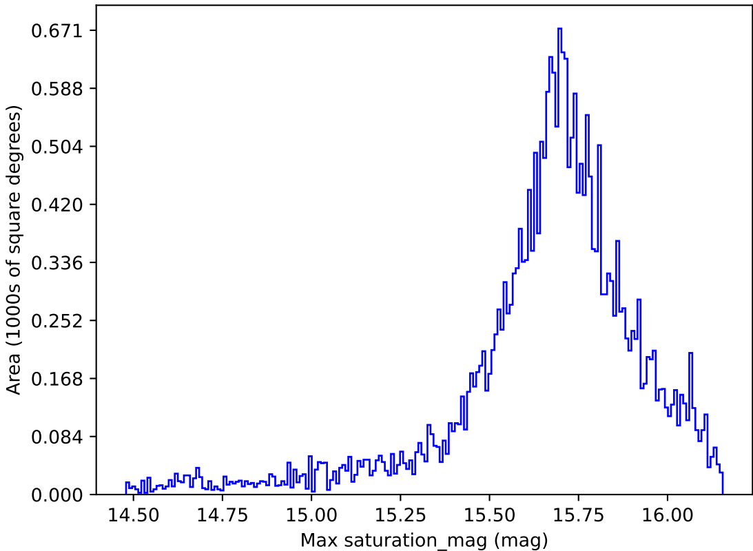
ddf_loaded_fl8_v3.4_10yrs All sky r band: Max saturation_mag
